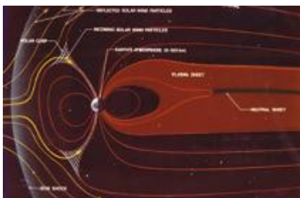
Space Weather [1]
